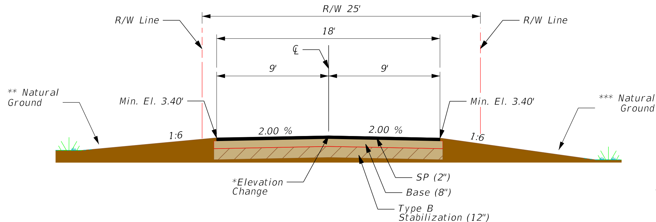
Typical Section 4
